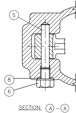
A-VIEW CAPTURED GASKET
