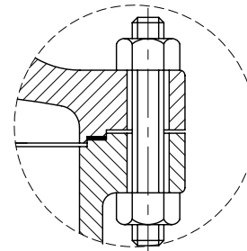
A-VIEW CAPTURED GASKET
